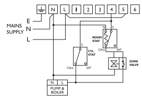
425 Coronet controlling fully pumped system via room stat, cylinder stat and using a 2 port spring return valve with auxiliary switch on heating circuit.
