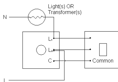
Figure 3 Using a 2-way Dimmerswitch
